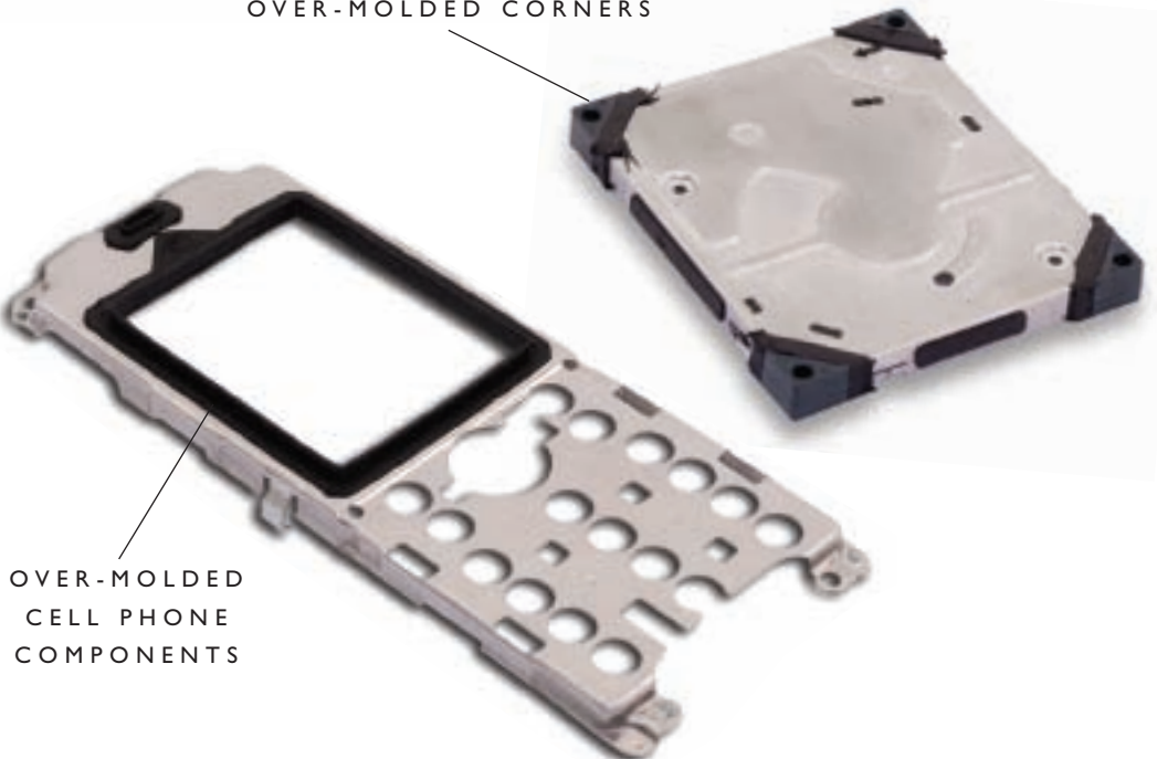
OVER-MOLDED CORNERS
