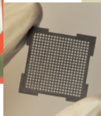
SOLDER COLUMN JIG FOR FBGA
